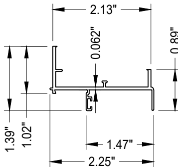
3G FRAME HEAD ALUM (6063-T6)
